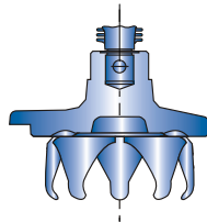
Throttling plug from DN 125
