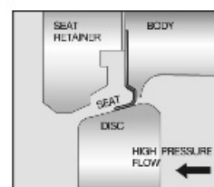
AFTER FIRE TEST
