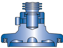
Throttling plug with PTFE seal ring, DN 15-100
