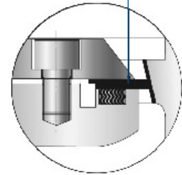
SEAT RING (Solid metal) 316SS+Nitr
