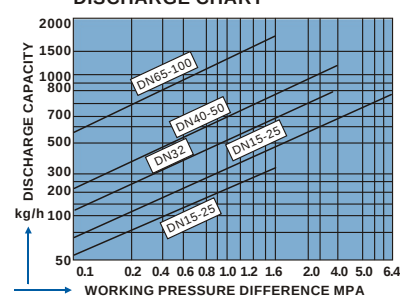
DISCHARGE CHART
