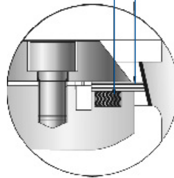
SPIRAL WOUND GASKET 316SS+Graphite
